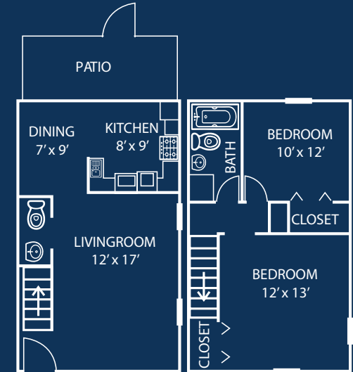
Two Bedroom/One & Half Bath (1000 Square Feet)
